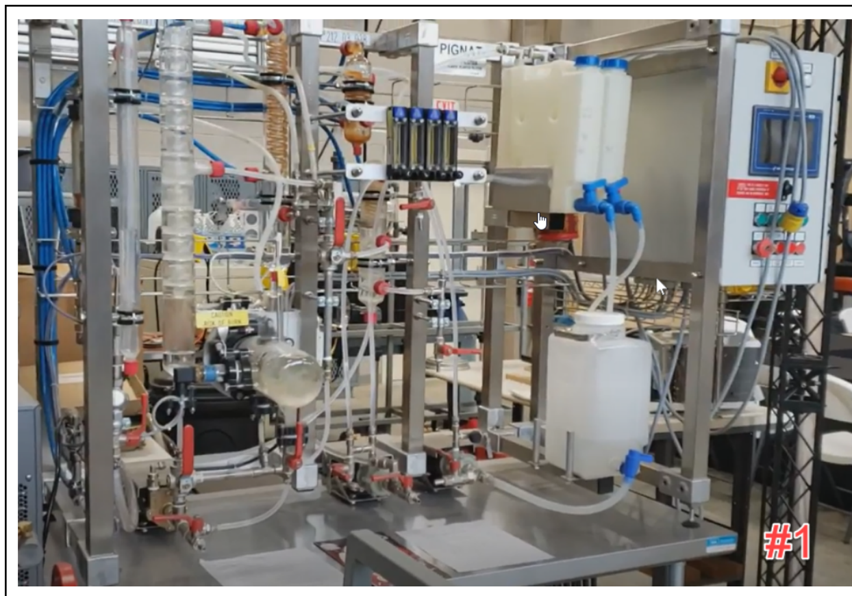
Distillation System training unit at South Ark CC.
