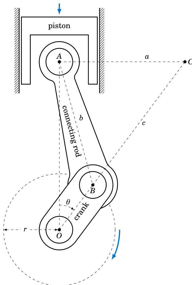
Figure 1.3.2 Slider-crank mechanism
