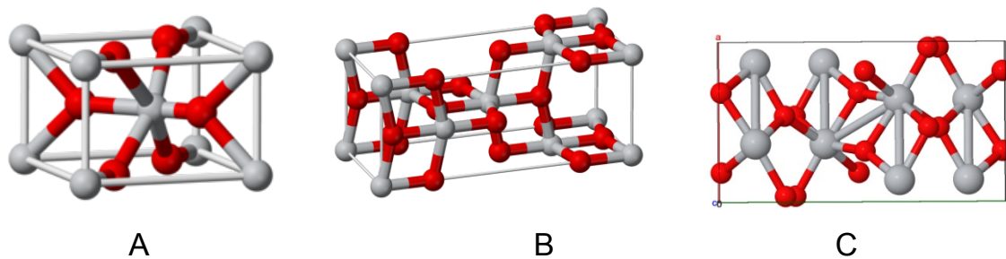
Figure 2. Representations of the crystal unit cells of titanium dioxide. (A) rutile, (B) anatase, (C) brookite. Images from www.labspace.net , Wikimedia Commons , and http://materials.springer.com .
