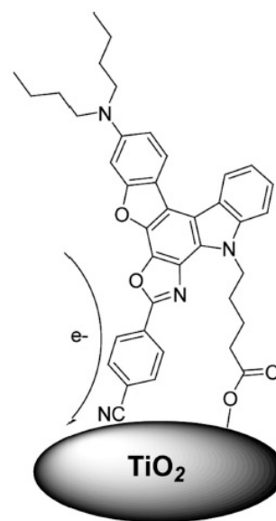
Figure 3. Molecular structure of one possible dye in a DSC. Image from Hagfeldt et al (2010) (Reference #3 of this module).
