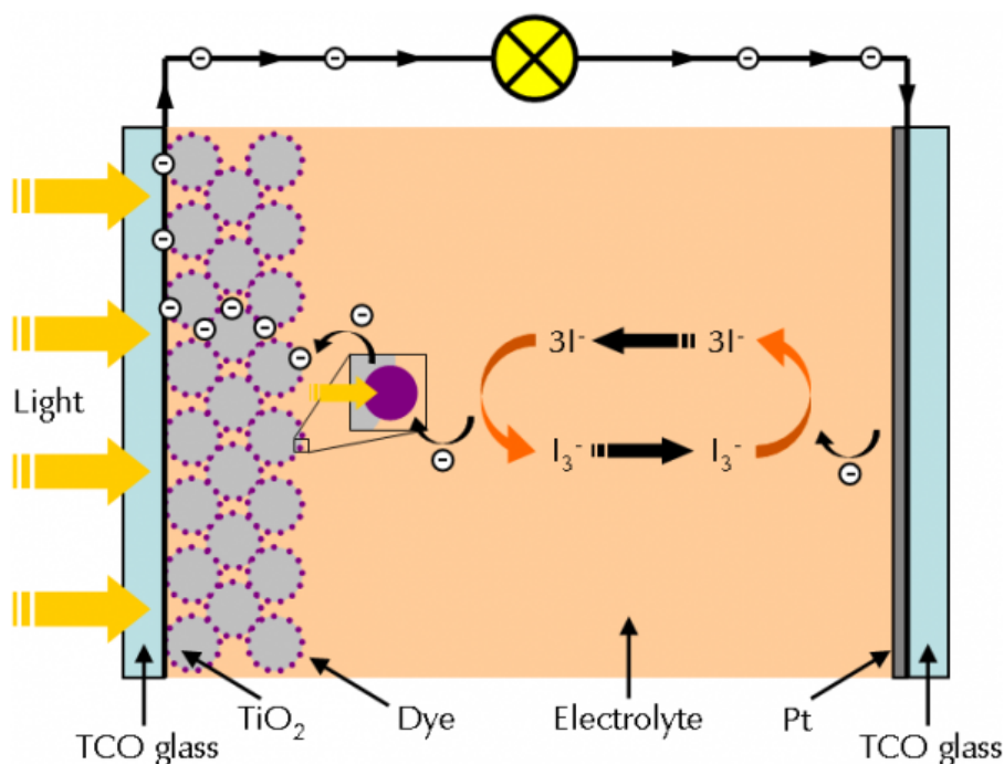
Figure 1. The structure of a dye-sensitized solar cell. From: Gamry.com.
