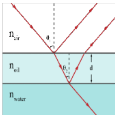
Figure 3. Constructive interference occurs when waves overlap in phase. Destructive interference happens when waves overlap out of phase.
